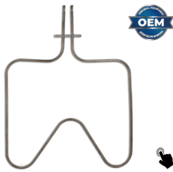
WA229 3871428011 Electrolux ITA Resistenza base forno 230v 1000 W ENG Lower oven heating element 1000 W 230V
