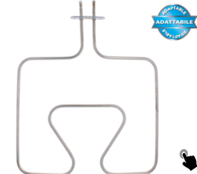
WA230 3970125013 Electrolux ITA Resistenza base forno 230v 1050 W adattabile ENG Lower oven heating element 1050 W 230V adaptable
