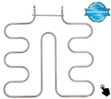
WA264 00688482 Bosch ITA Resistenza forno superiore 1200 W adattabile ENG Upper oven heating element 1200 W 230V adaptable
