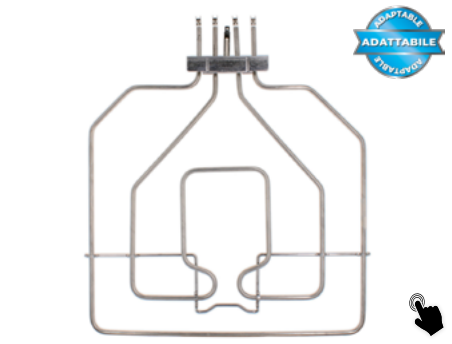
WA242 470845 Bosch ITA Resistenza superiore forno 230v 1500+1300 W adattabile ENG Upper oven heating element 1500+1300 W 230V adaptable
